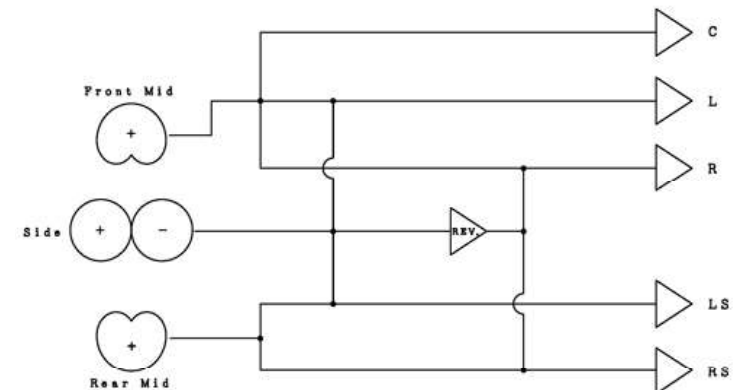
WMS-5 Block Diagram
